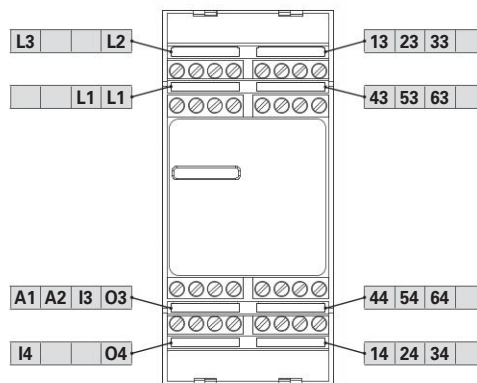
Terminal layout - CS AM23
