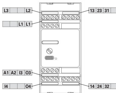
Terminal layout - CS AM14
